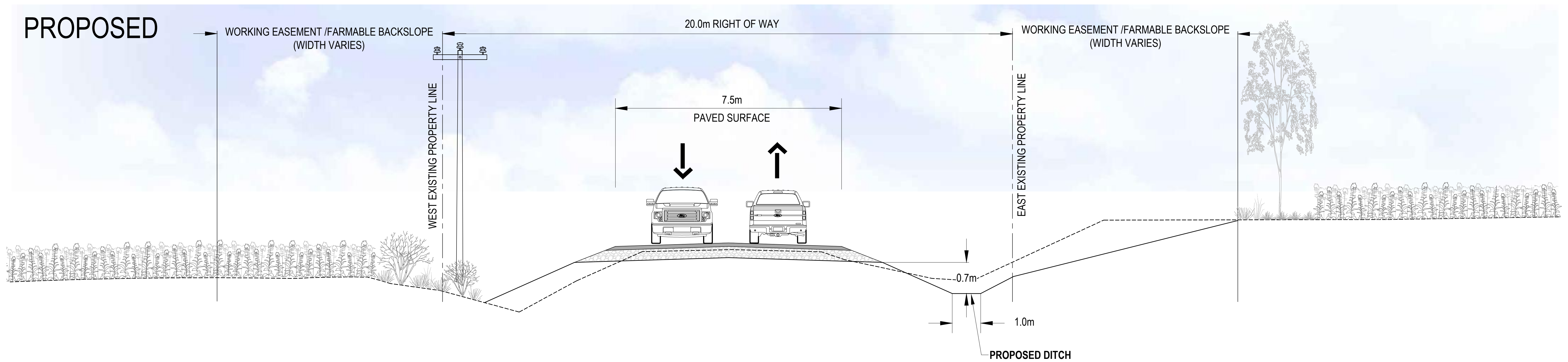
TYPICAL CROSS SECTION - PROPOSED RANGE ROAD 210
