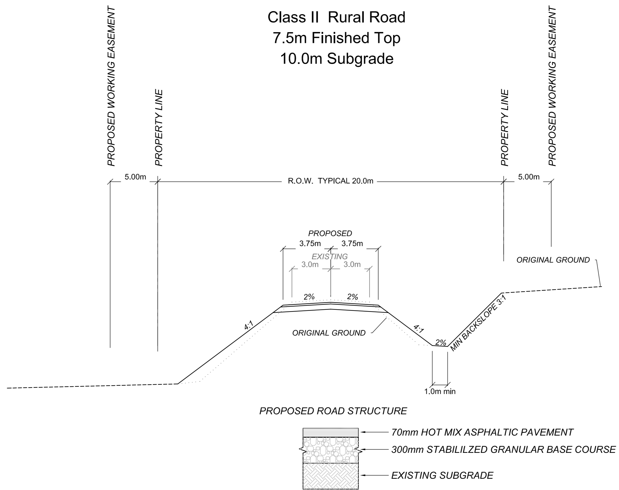
DETAIL 1 STANDARD CROSS SECTION - RANGE ROAD 213
