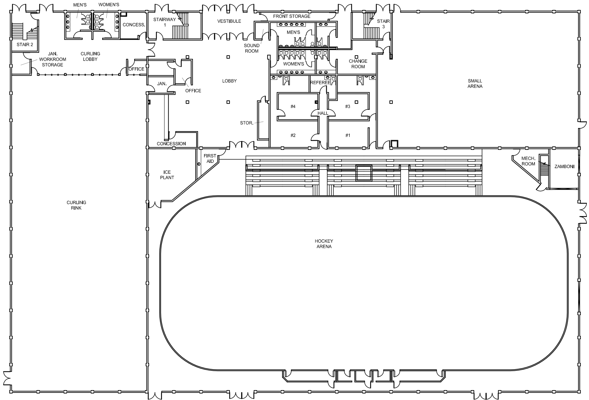
1 MAIN FLOOR PLAN A1
