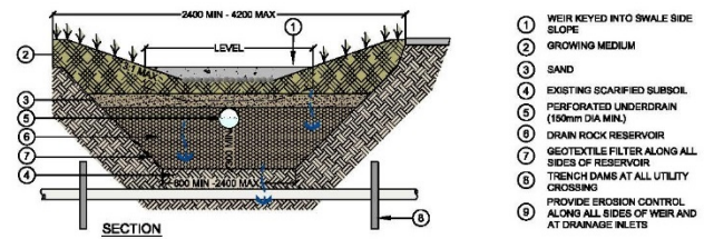
3 PARTIAL INFILTRATION SWALE WITH RESERVOIR AND SUBDRAIN D Not To Scale Plan / Section
