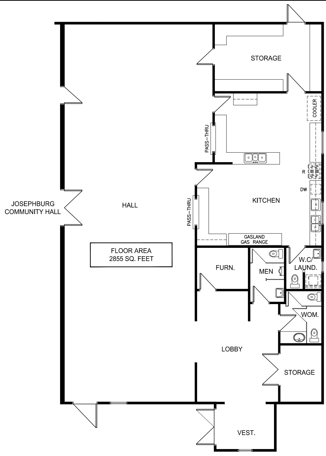
1 MAIN FLOOR PLAN A1 1/8" = 1'-0"
