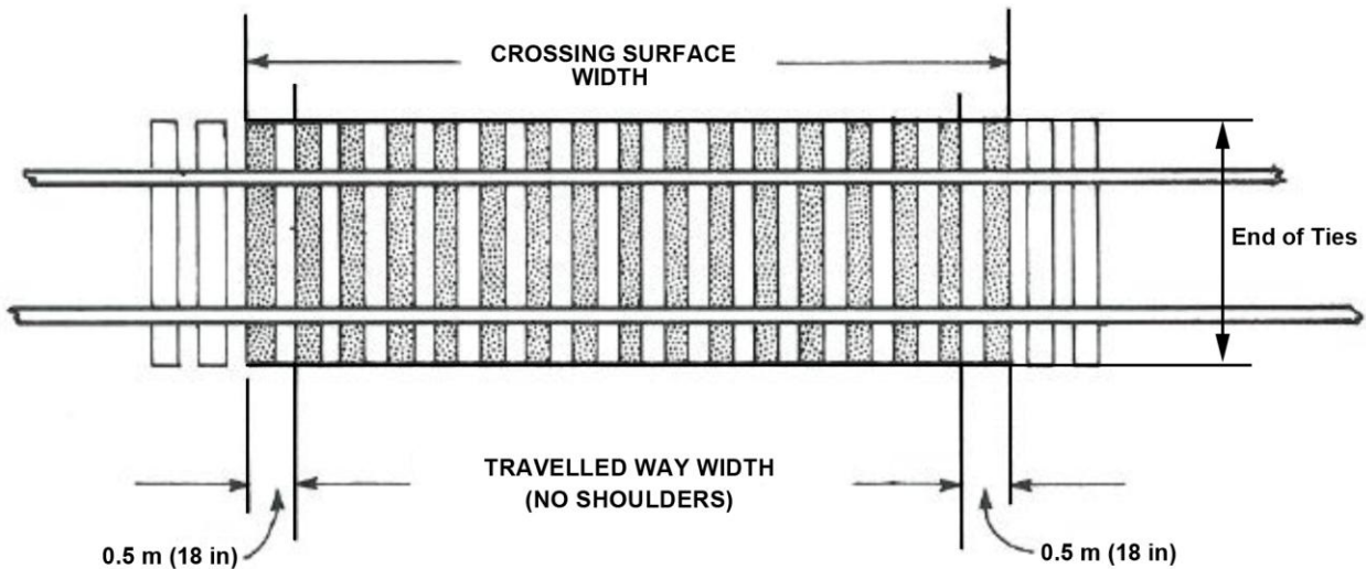
Figure 3-1 – Crossing Surface
