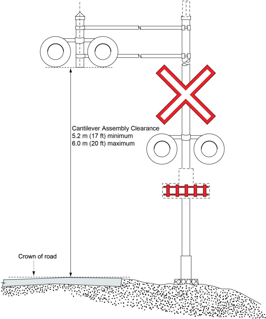
Figure 12-3 – Cantilevers
